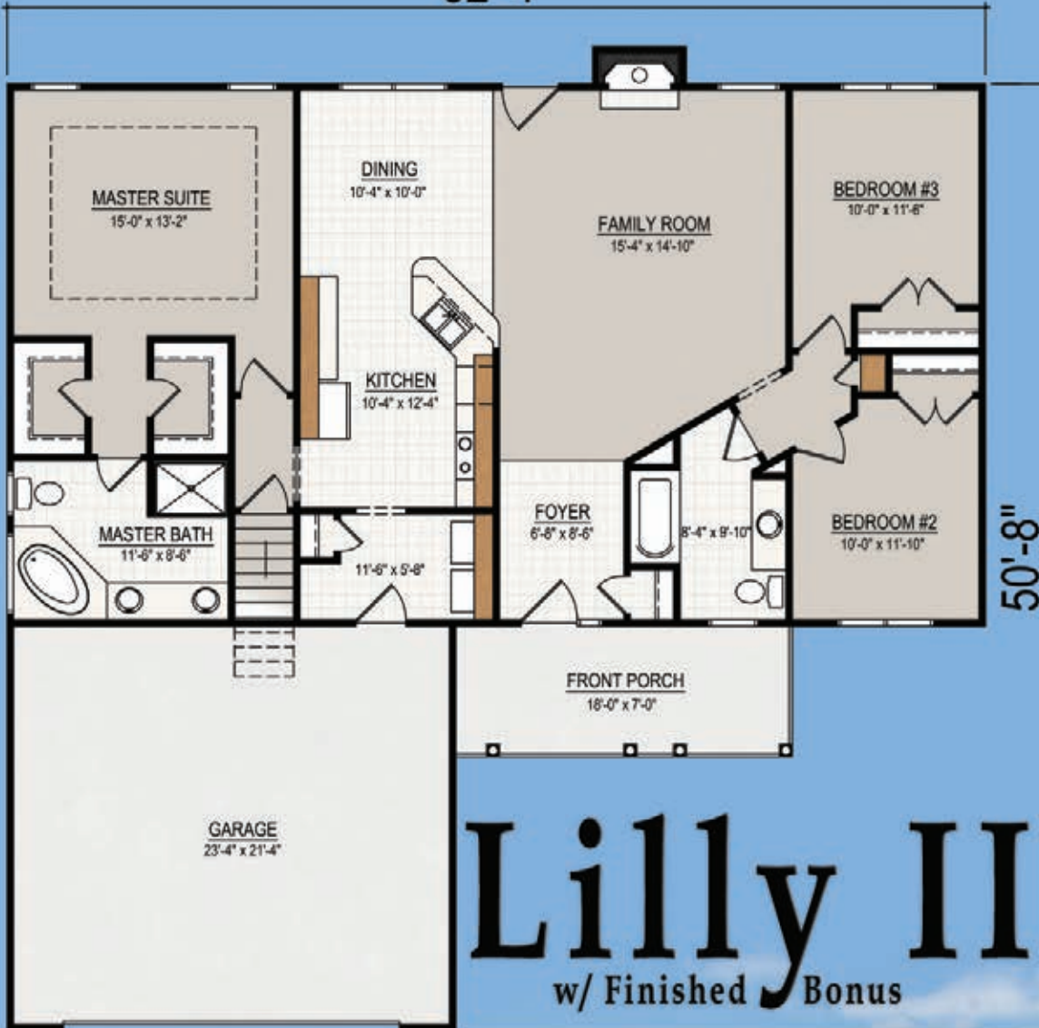
FIRST FLOOR PLAN CEILING HT. = 8'-0"
