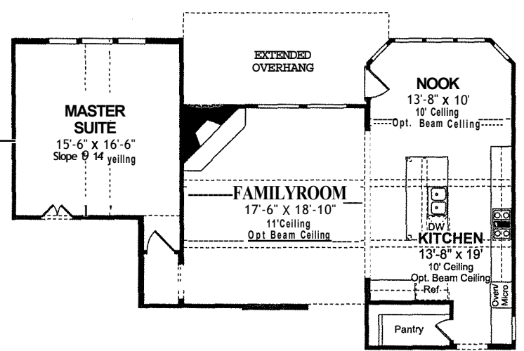
OPT. FAMILY ROOM EXTENSION
