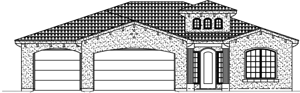
FRONT ELEVATION (OPTION "B")
