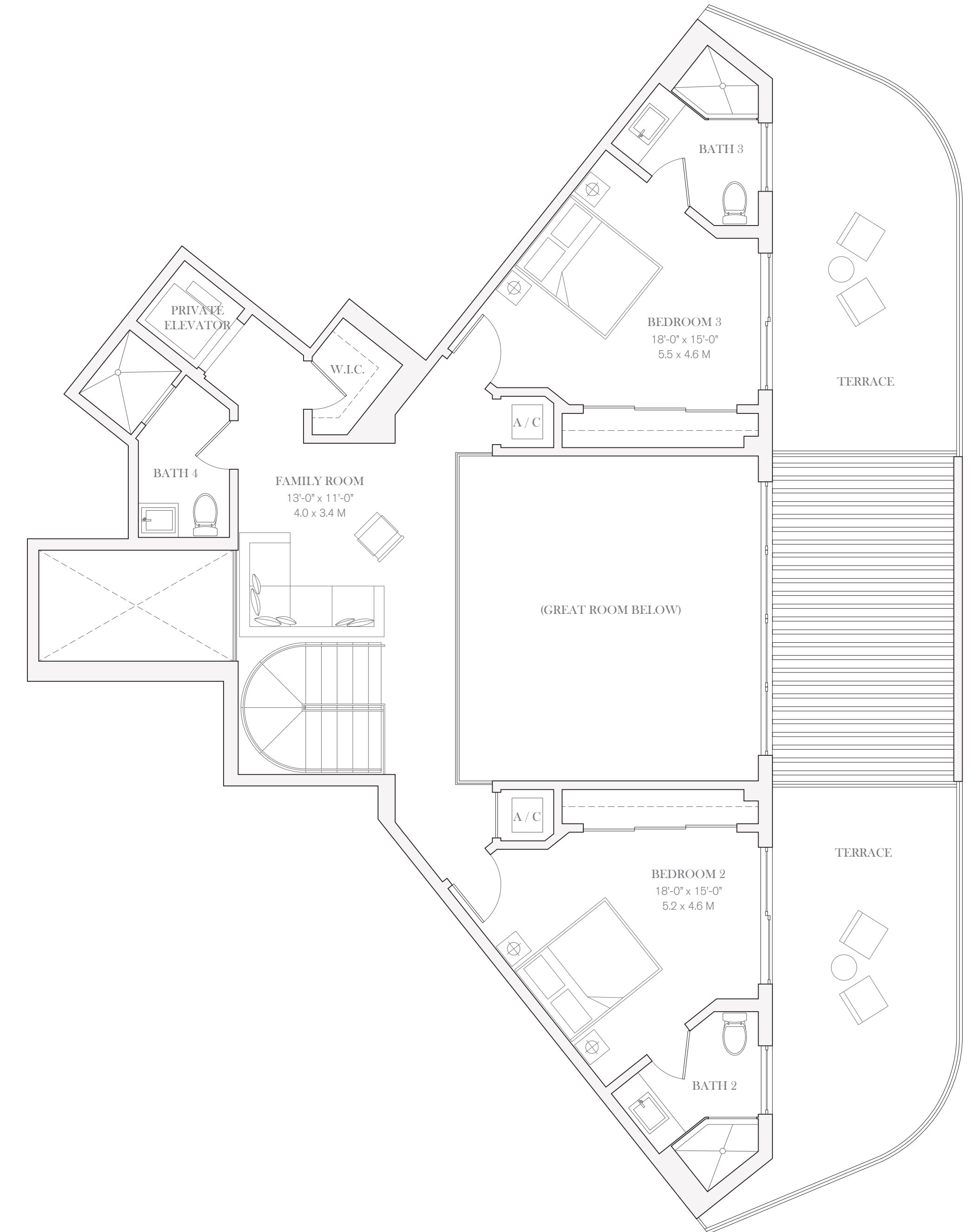
UPPER LEVEL
