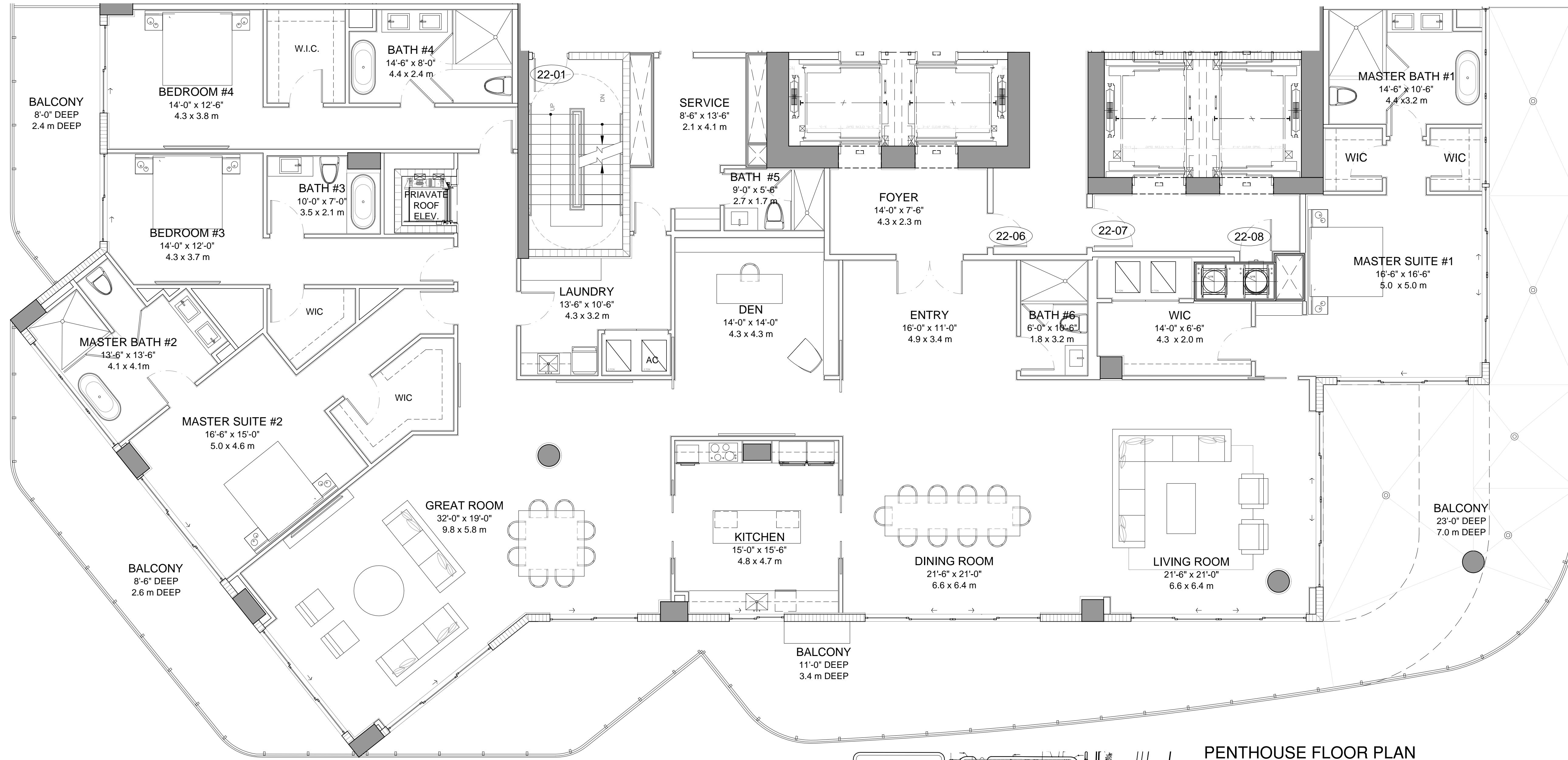
PENTHOUSE FLOOR PLAN LEVEL 22 3/16" = 1'-0"
