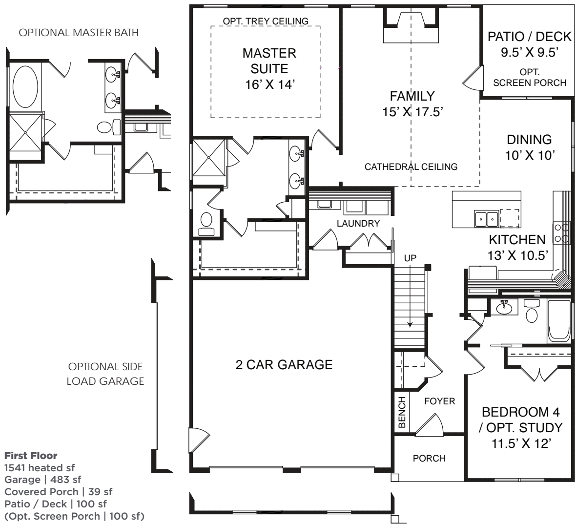
FIRST FLOOR
